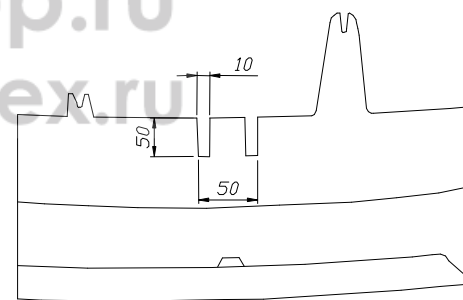
Fig. 3 Bumper cut.
